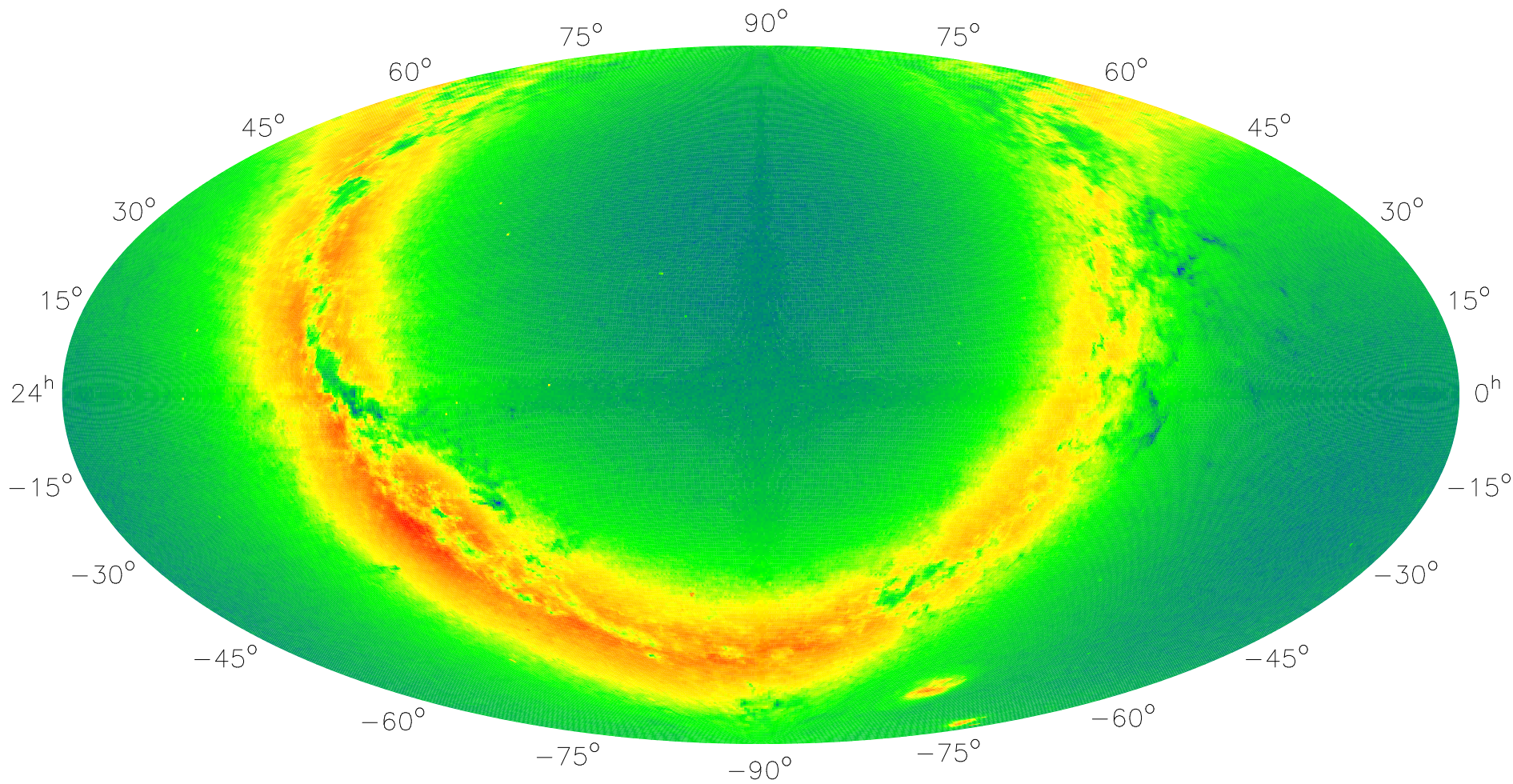
UCAC4 log total numb.stars/box of 0.5 deg
